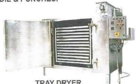
TRAY DRYER
